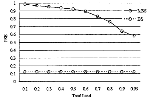
Fig. 5. PSE of LBPS-merge with PSE\_TH = 0.125
