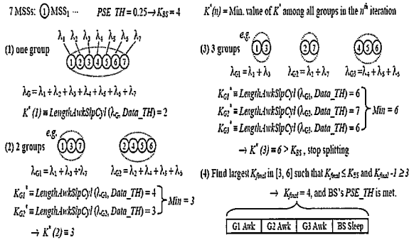
Fig. 1. An example of LBPS-split under S2.
