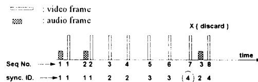
Fig. 7d. video advance ( audio delay )
